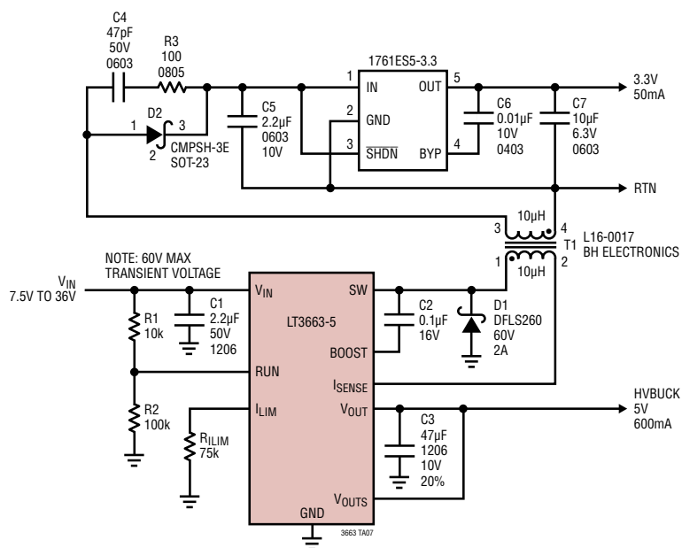
LT3663-5 5V Step-Down Regulator with Isolated 3.3V Output
