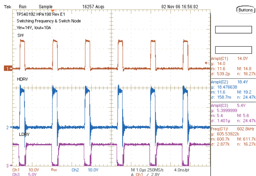
Figure 8. TPS40192EVM-001 Switching Waveforms, CH1: SW(TP), CH2: HDRV(TP), CH3: LDRV(TP); Vin = 14 V, Vout = 1.8 V, Iout = 10 A
