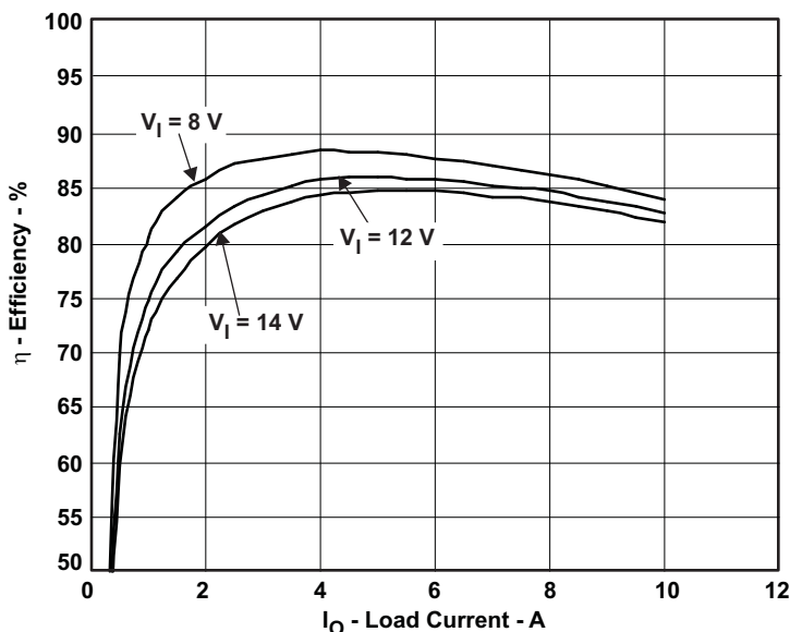
Figure 4. TPS40192EVM-001 Efficiency vs Load Current, V_{in} = 8 \text{ V} - 14 \text{ V} , V_{out} = 1.8 \text{ V} , I_{out} = 0 \text{ A} - 10 \text{ A}
