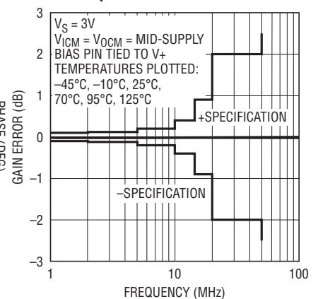
Gain Error Relative to 1MHz vs Temperature
