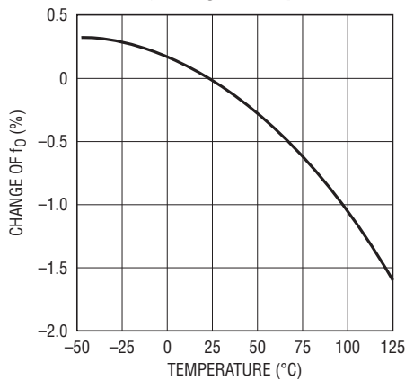
% Change of f 0 vs Temperature
