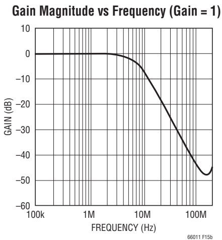
Figure 15. Modified Filter Configuration Using a Resistor Between Summing Nodes ( f_{-3dB} = 7.5\text{MHz} )
