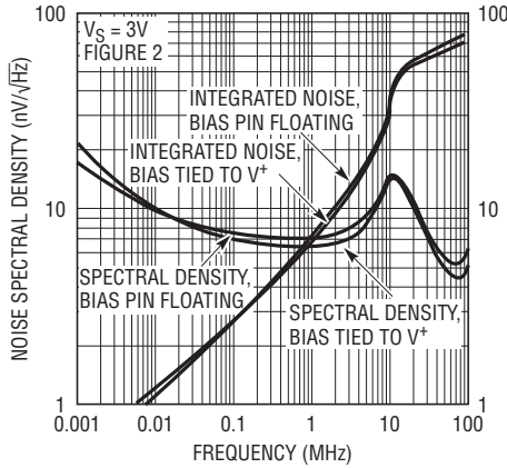
Differential Output Noise
