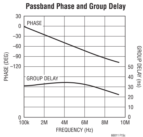
Figure 15. Modified Filter Configuration Using a Resistor Between Summing Nodes ( f_{-3dB} = 7.5\text{MHz} )
