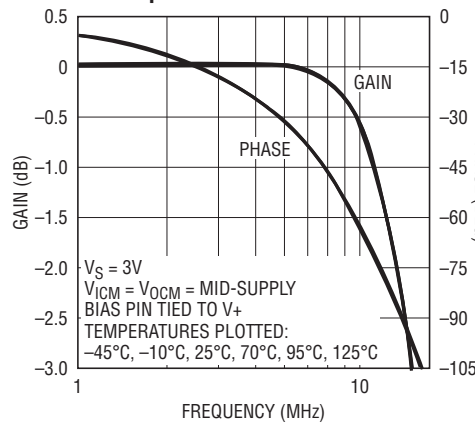
Passband Gain and Phase vs Temperature
