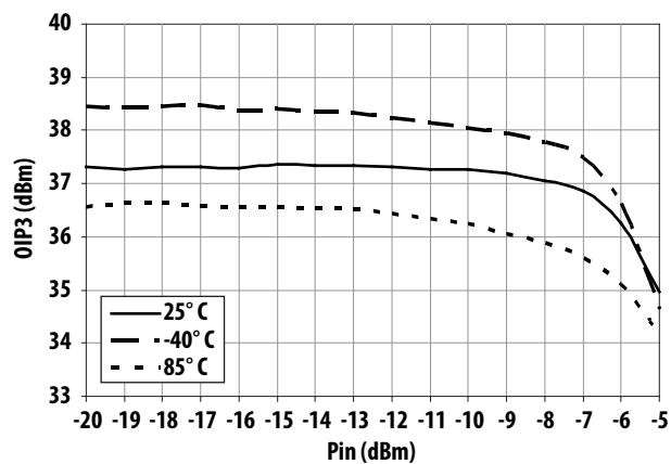
Figure 23. OIP3 vs Input Power and Temperature
