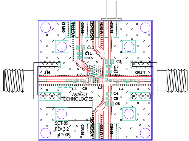
Figure 26. Demoboard
