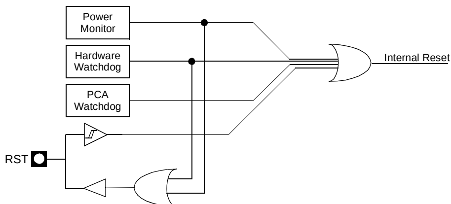
Figure 9. Reset schematic
