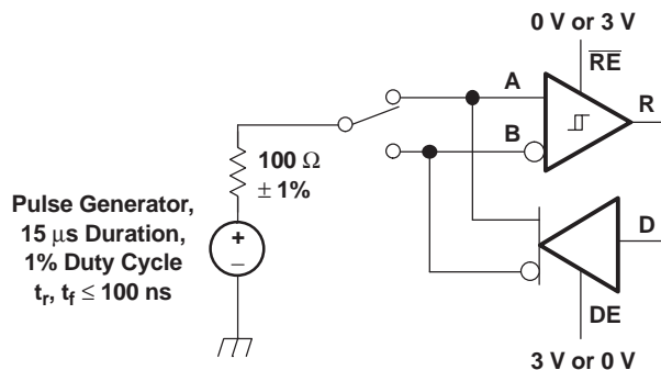
Figure 20. Test Circuit, Transient Overvoltage Test
