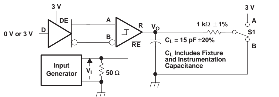
Figure 17. Receiver Switching Test Circuit and Voltage Waveforms
