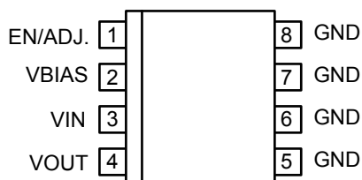
8-Pin Power MSOP (MM)
