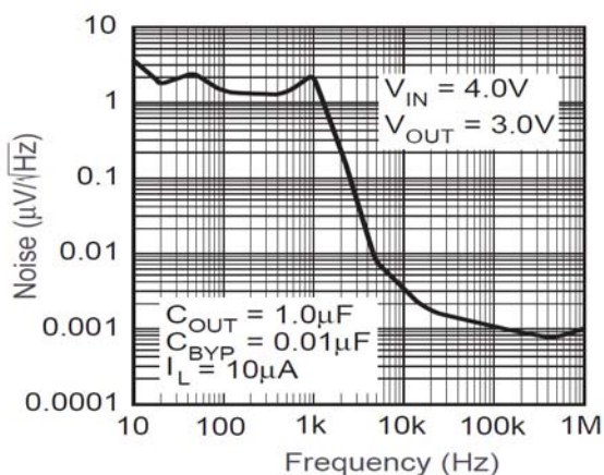
Figure 11. Noise Performance
