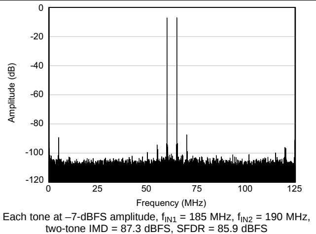
Figure 22. FFT for Two-Tone Input Signal
