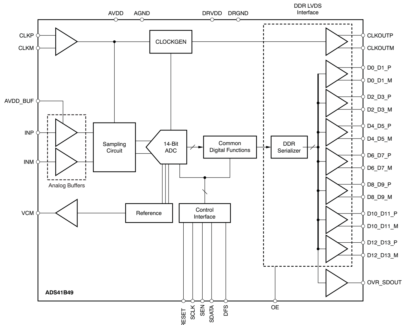
Figure 53. ADS41B49 Block Diagram
