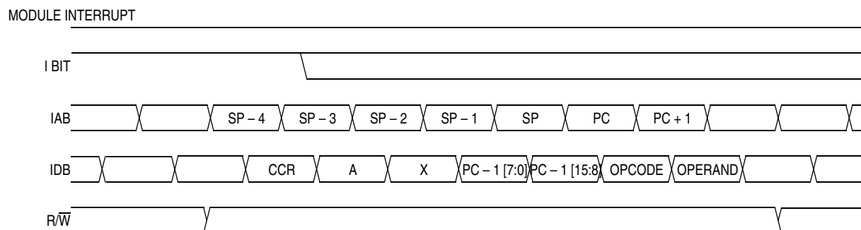
Figure 15-10. Interrupt Recovery
