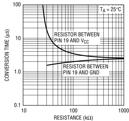
Conversion Time vs R_{EXT}
