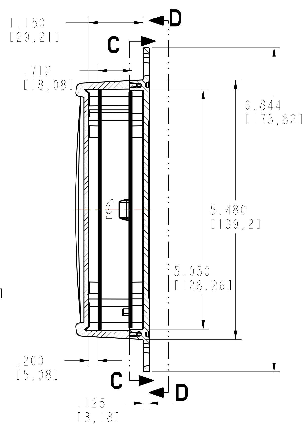
SECTION B-B
