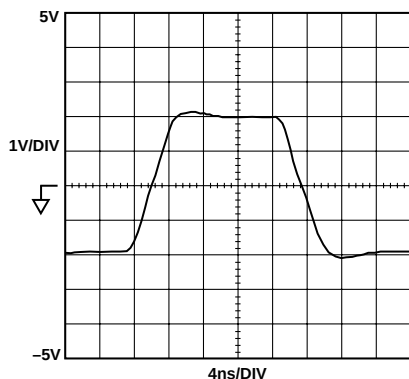
Figure 17. Large Signal Step Response G = -1 , R_L = 1 \text{ k}\Omega
