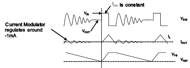
Figure : Light-Load Operation
