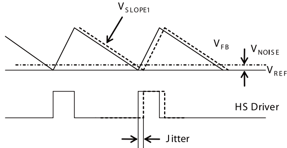
Figure : Jitter in PWM Mode
