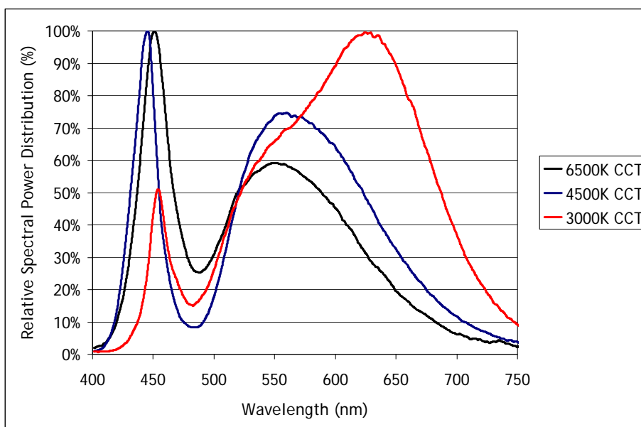
Typical Relative Spectral Power (T J = 25°C)
