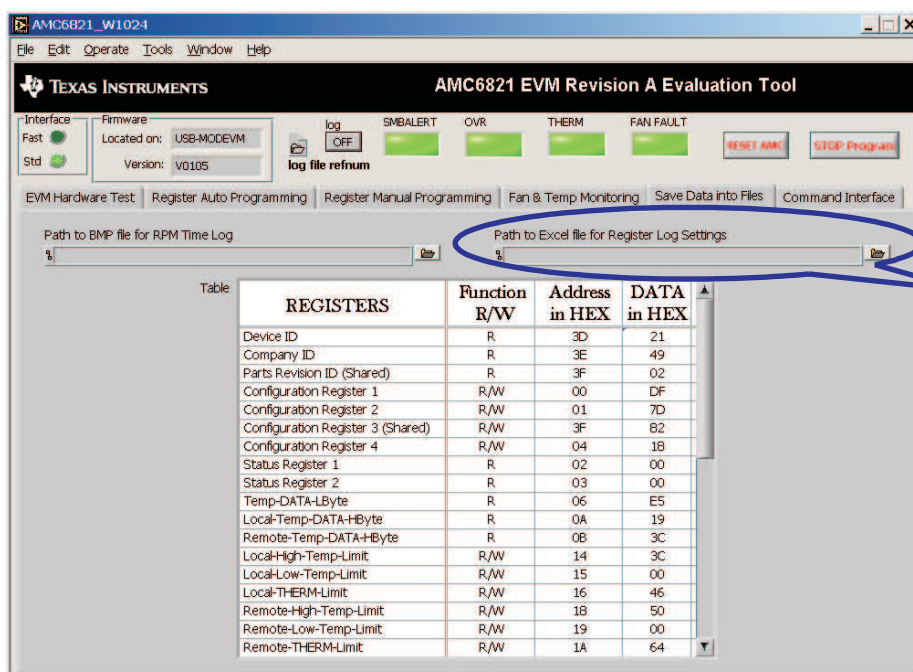
Figure 19. Register Settings
