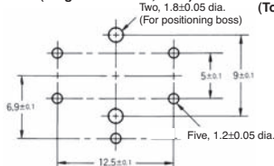
PCB Mounting (Top View) (Single-sided PCB, t \leq 1.6 )
