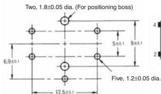
PCB Mounting (Top View) (Single-sided PCB, t \leq 1.6 )
