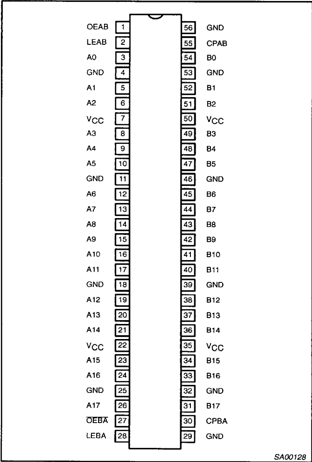
PIN CONFIGURATION
