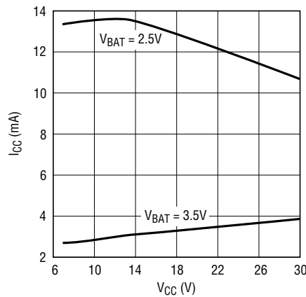
I_{\text{CC}} vs V_{\text{CC}} (4.2V Version)
