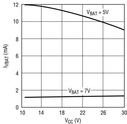
I_{\text{VBAT}} vs V_{\text{CC}} (8.4V Version)
