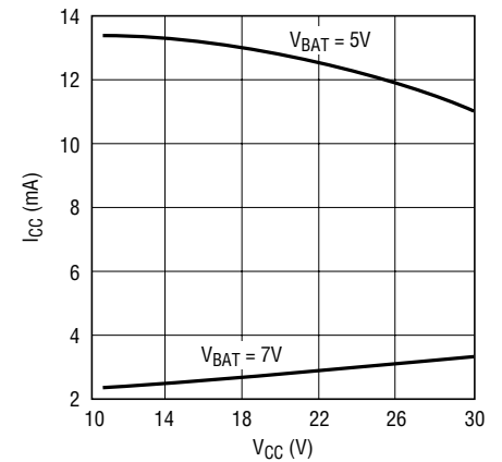
I_{\text{CC}} vs V_{\text{CC}} (8.4V Version)
