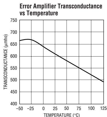
LT1776 G12
