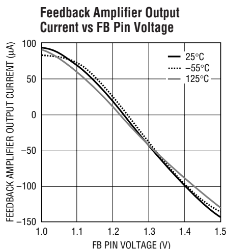
LT1776 G11
