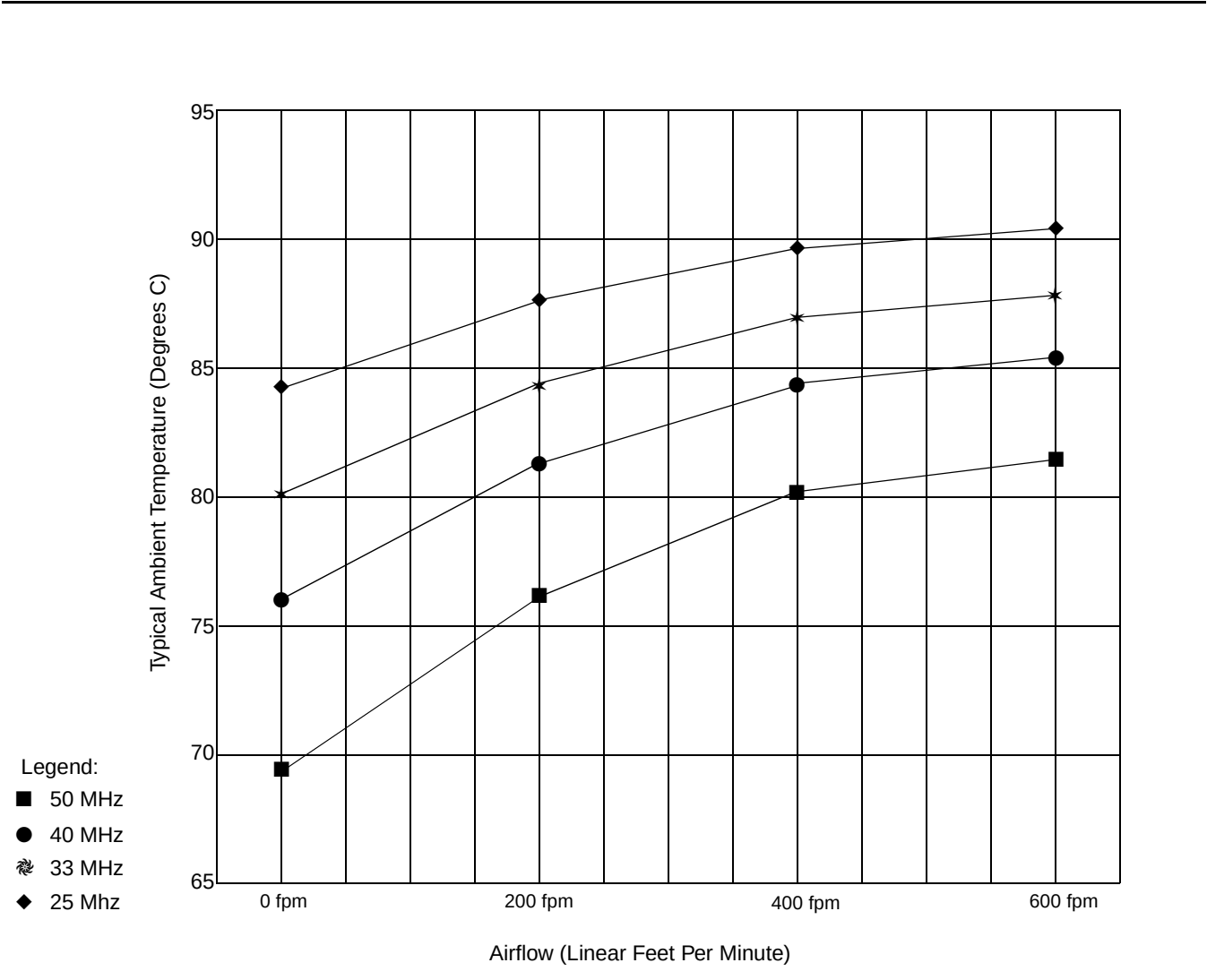
Figure 19. Typical Ambient Temperatures for TQFP with Two-Layer Board
