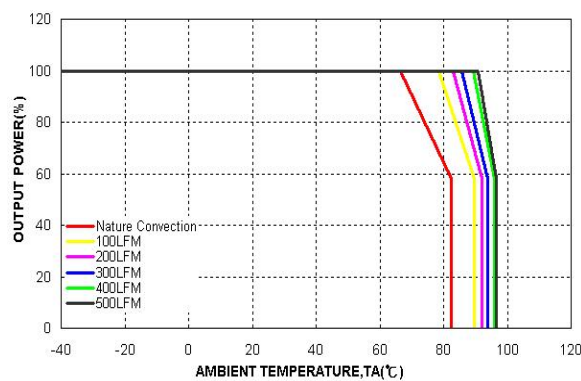
Derating Output Current Versus Ambient Temperature with Heat-Sink and Airflow, V_{in} = V_{in\ nom}
