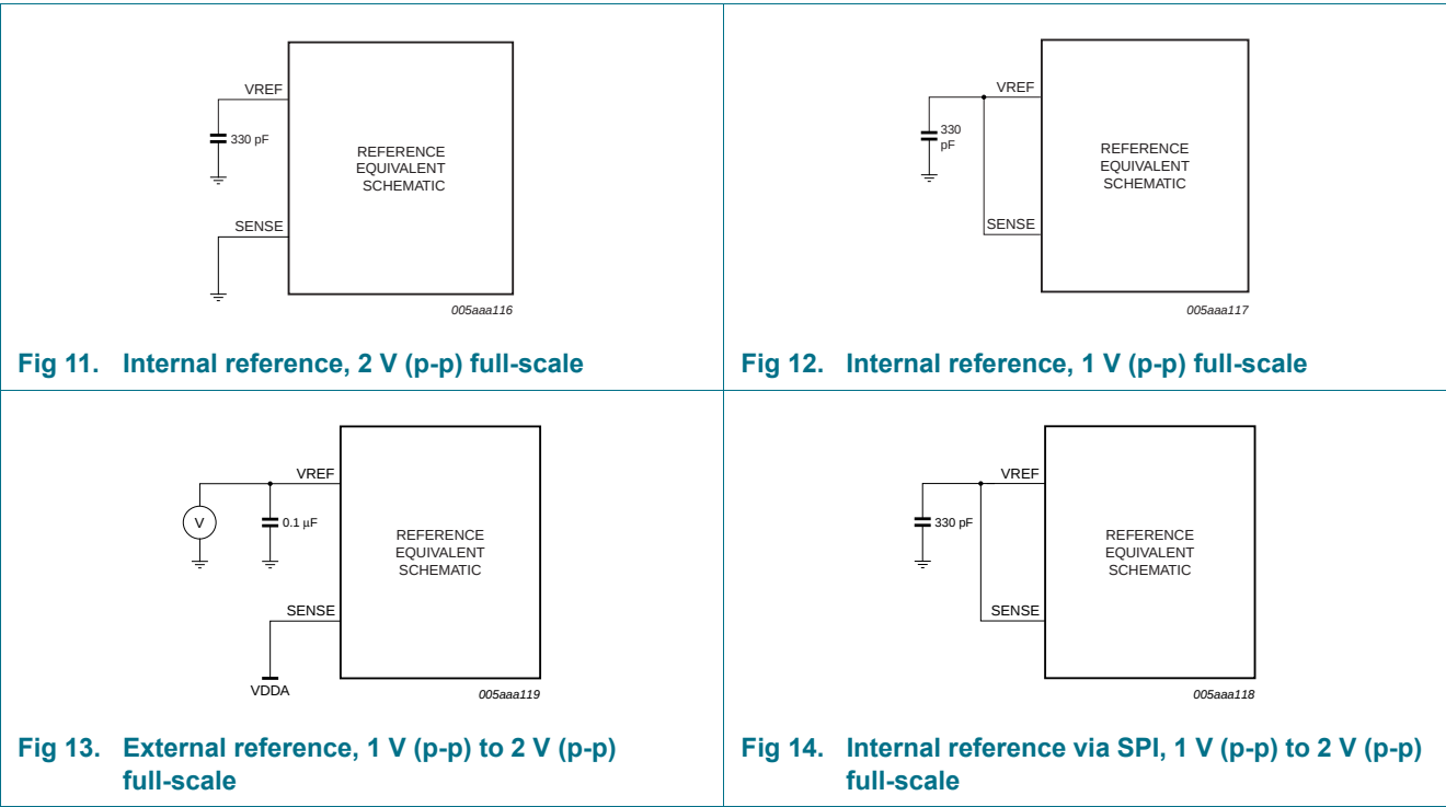
Figure 11 to Figure 14 illustrate how to connect the SENSE and VREF pins to select the required reference voltage source.
