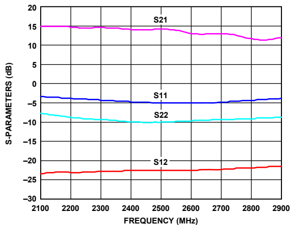
Figure 15. Typical S-Parameters, Log Magnitude
