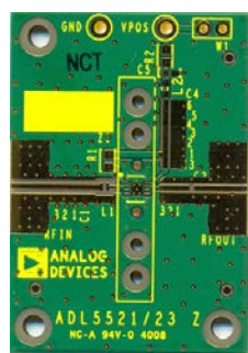
Figure 55. Evaluation Board Layout (Top View)
