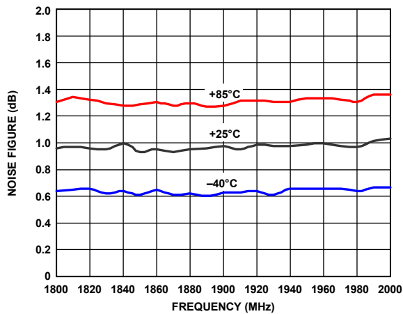
Figure 35. Noise Figure vs. Temperature
