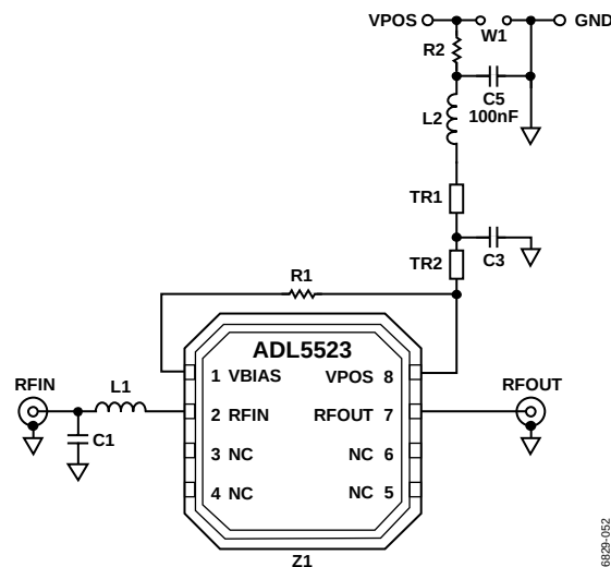
Figure 53. ADL5523 Basic Connections
