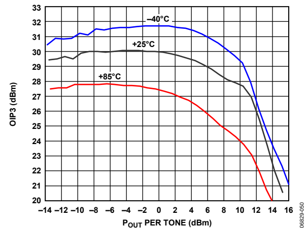
Figure 50. OIP3 vs. Output Power (P OUT ) and Temperature
