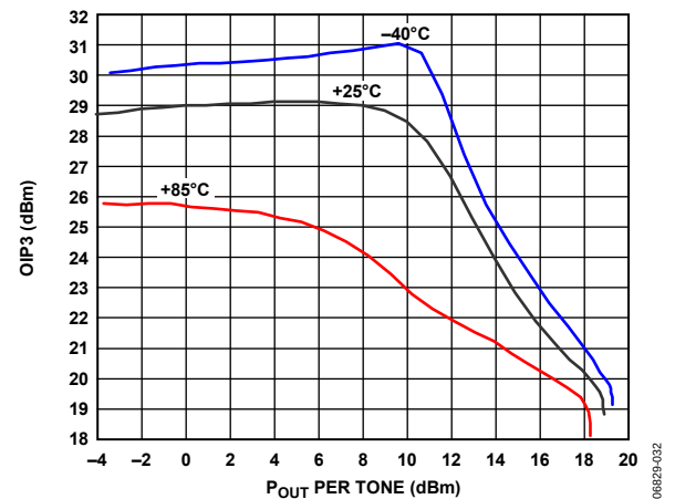
Figure 32. OIP3 vs. Output Power (P OUT ) and Temperature
