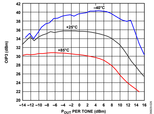
Figure 26. OIP3 vs. Output Power (P OUT ) and Temperature
