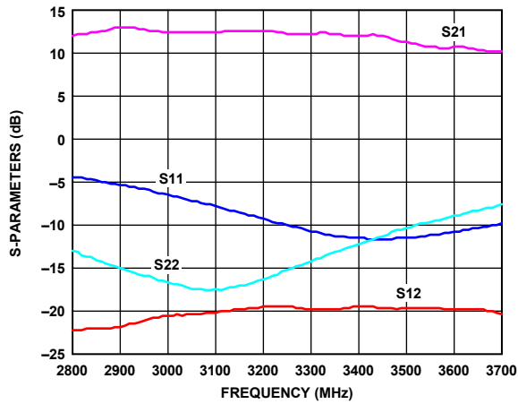
Figure 21. Typical S-Parameters, Log Magnitude
