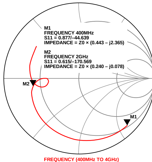
Figure 63. S11 of ADL5523 with S22 Matched at 2 GHz
