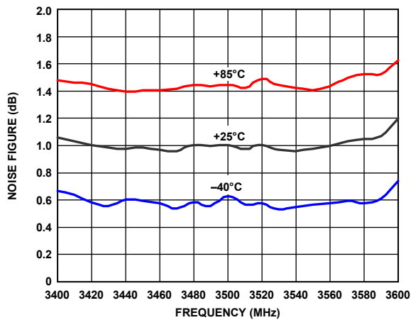
Figure 23. Noise Figure vs. Temperature
