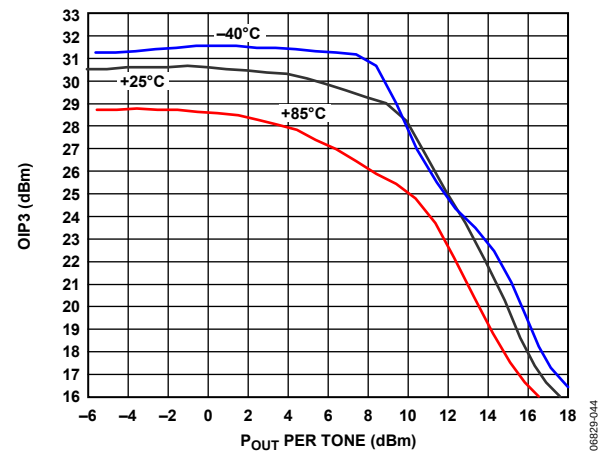
Figure 44. OIP3 vs. Output Power (P OUT ) and Temperature
