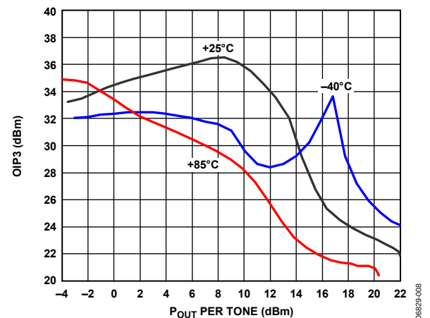
Figure 8. OIP3 vs. Output Power ( P_{OUT} ) and Temperature
