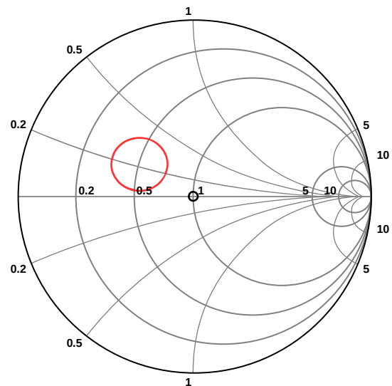
Figure 61. Area of Optimal Noise Matching for ADL5523
