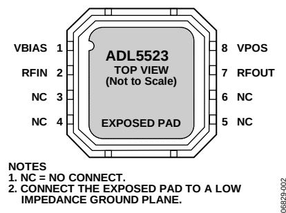
Figure 2. Pin Configuration
