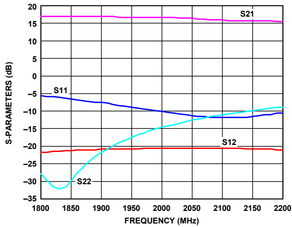
Figure 33. Typical S-Parameters, Log Magnitude
