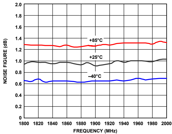
Figure 11. Noise Figure vs. Temperature
