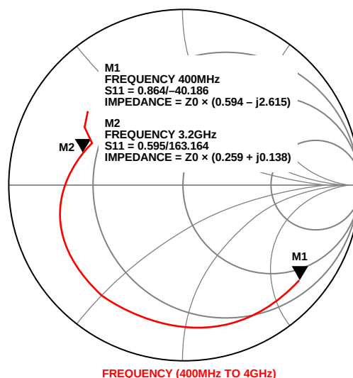
Figure 64. S11 of ADL5523 with S22 Matched at 3.2 GHz
