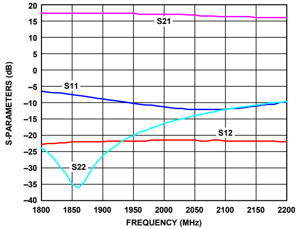
Figure 9. Typical S-Parameters, Log Magnitude
