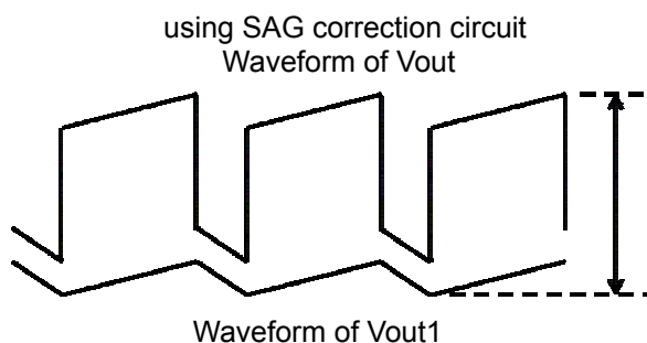
Waveform of Vout terminal and Vout1 terminal
