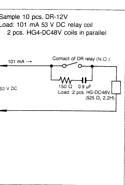
Electrical life test
