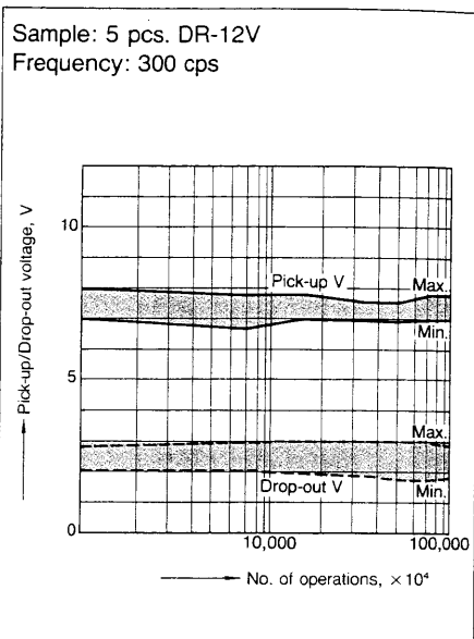
Electrical life
