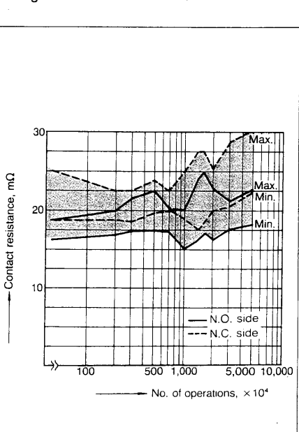
Change of contact resistance
