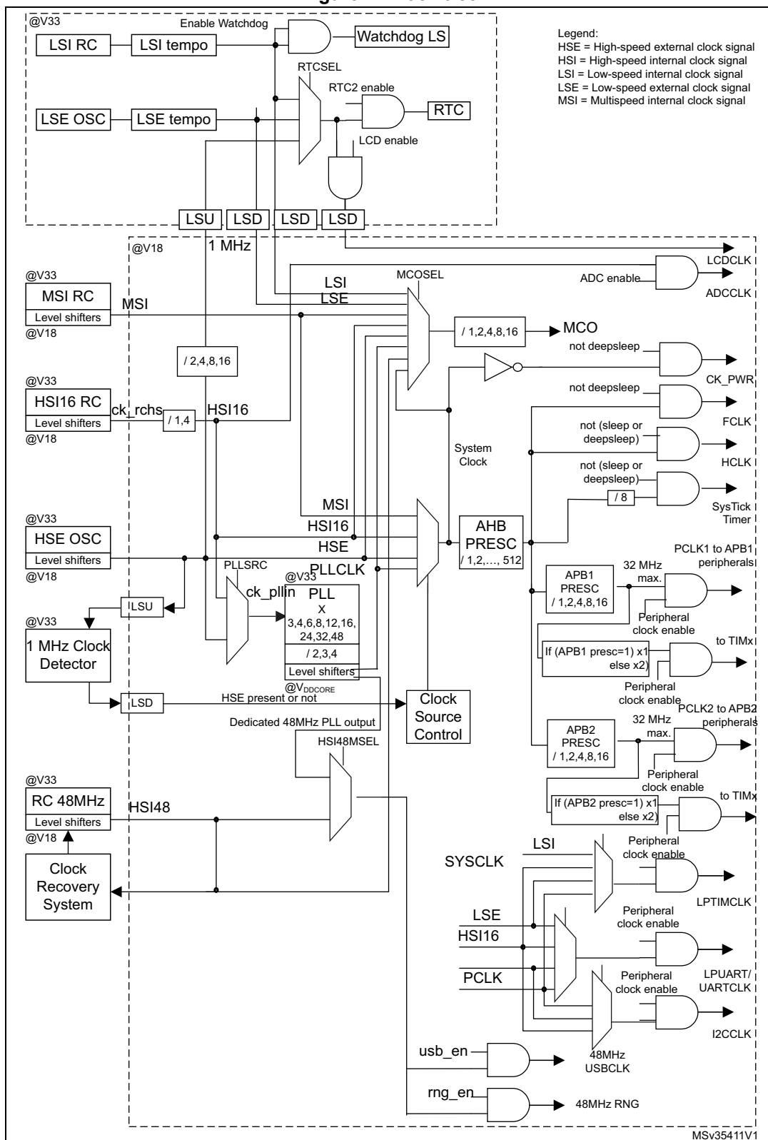
Figure 2. Clock tree
