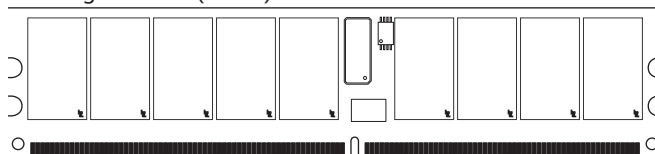
Figure 1: 240-Pin DIMM (MO-237 R/C G)
