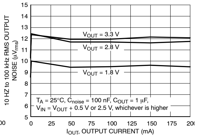
Figure 25. Output Noise vs. Load Current, C_{\text{noise}} = 100 \text{ nF} , C_{\text{OUT}} = 1 \mu\text{F}
