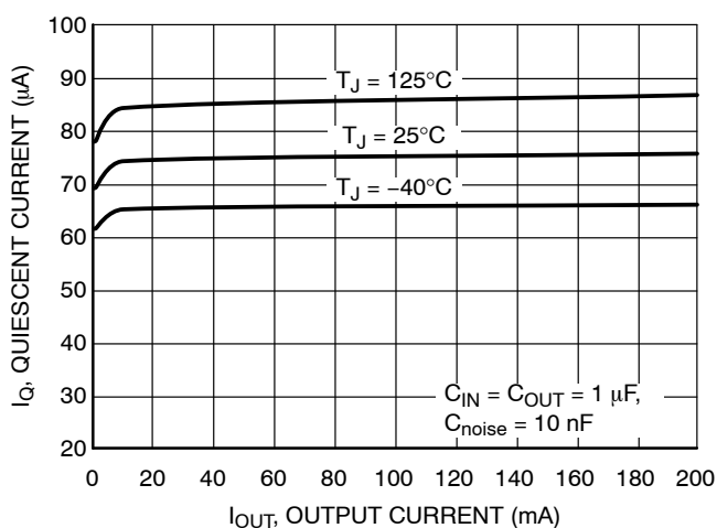
Figure 54. Quiescent Current vs. Output Current, V_{OUT} = 2.8\text{ V}
