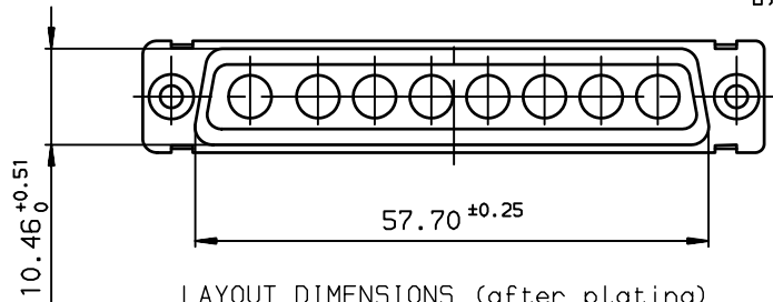
LAYOUT DIMENSIONS (after plating) CONNECTOR SIDE VIEW
