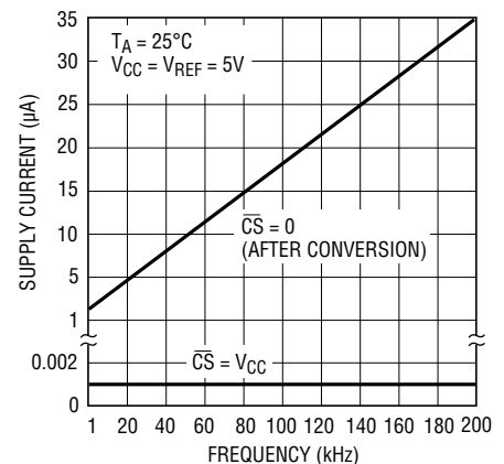
Shutdown Supply Current vs Clock Rate with \overline{\text{CS}} High and \overline{\text{CS}} Low
