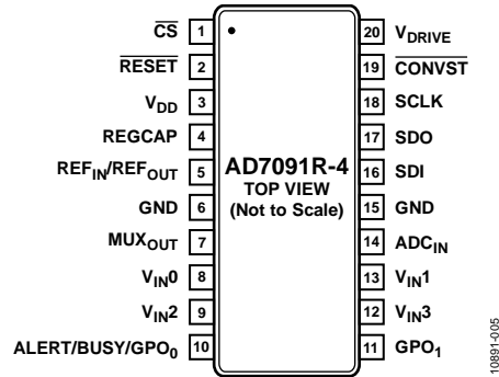
Figure 6. 4-Channel Pin Configuration
