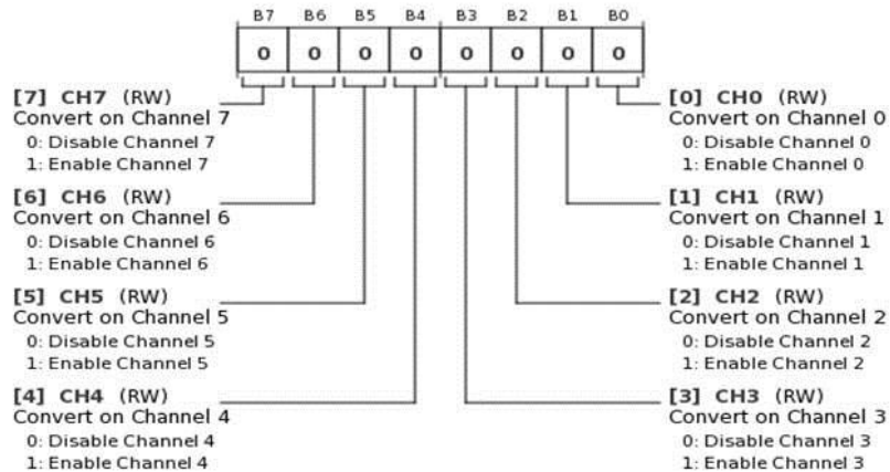
Figure 44. Channel Registers
