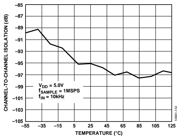
Figure 33. Channel-to-Channel Isolation vs. Temperature
