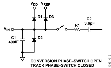
Figure 40. Equivalent Analog Input Circuit
