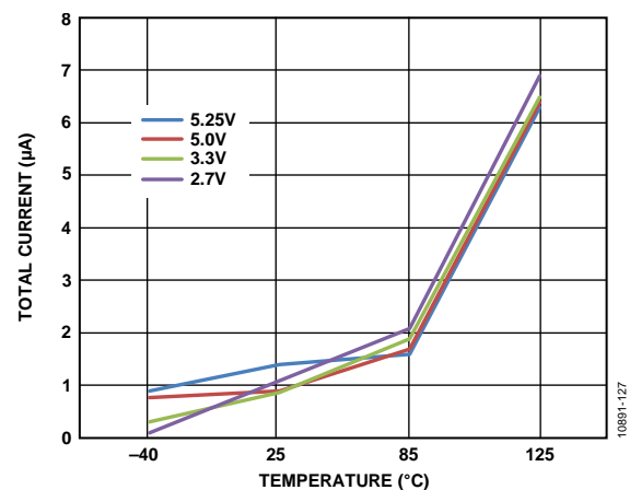
Figure 25. Total Power-Down Current vs. Temperature for Various Supplies
