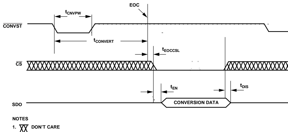
Figure 49. Serial Interface Read Timing in Normal Mode
