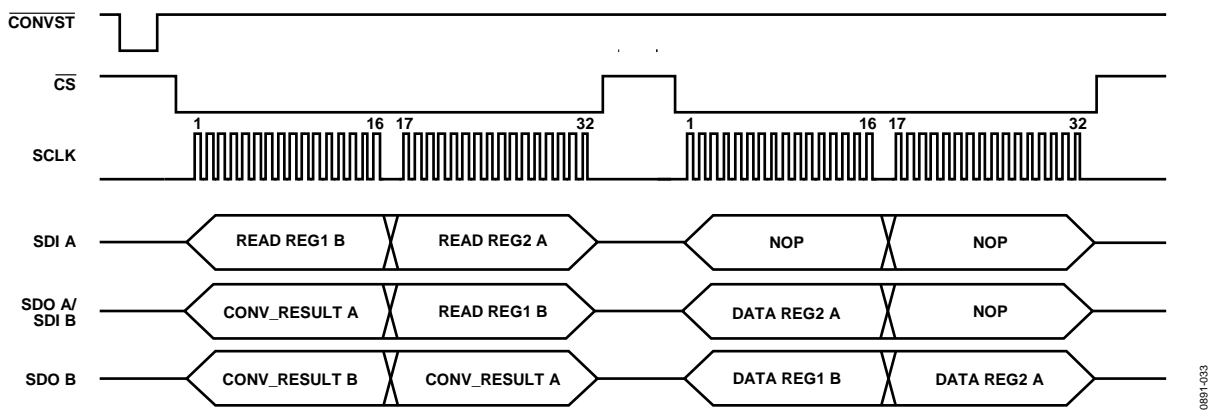
Figure 55. Single Register Read in a Two-Slave Daisy-Chain Mode Configuration
