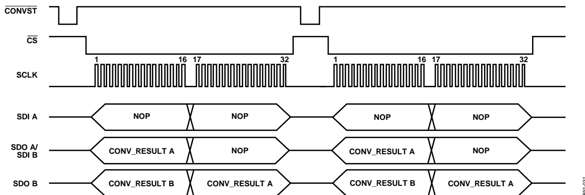
Figure 53. Conversion in a Two-Slave Daisy-Chain Mode Configuration
