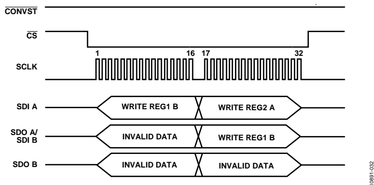
Figure 54. Single Register Write in a Two-Slave Daisy-Chain Mode Configuration
