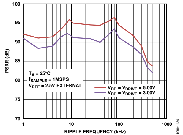
Figure 29. PSRR vs. Ripple Frequency
