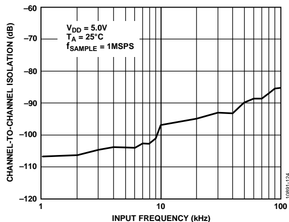
Figure 32. Channel-to-Channel Isolation vs. Input Frequency
