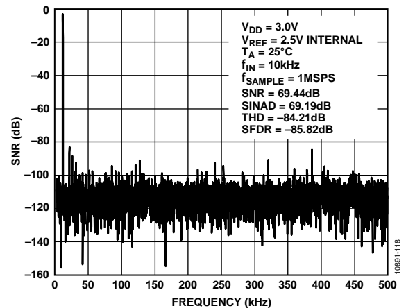
Figure 13. 10 kHz FFT, V_{DD} = 3.0\text{ V} , V_{REF} = 2.5\text{ V} Internal
