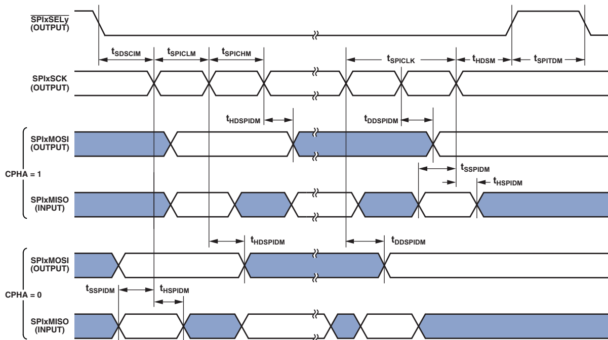
Figure 26. Serial Peripheral Interface (SPI) Port—Master Timing
