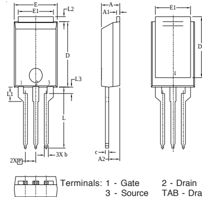
PLUS220 (IXTV) Outline
