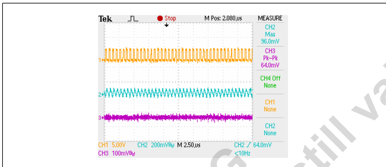
Figure 28. sdX_dis_curmin=1 operation
