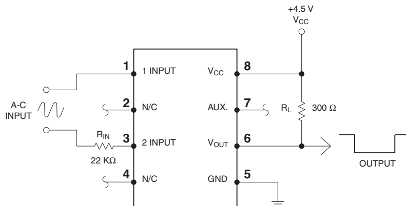
TEST CIRCUIT
