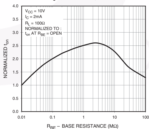
Fig. 6 Normalized t_{on} vs. RBE
