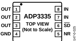
Figure 4. 8-Lead LFCSP
