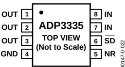
Figure 3. 8-Lead MSOP
