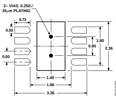
Figure 25. 3 mm x 3 mm LFCSP Pad Pattern (Dimensions shown in millimeters)
