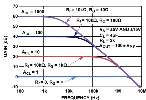
FIGURE 24. FREQUENCY RESPONSE vs CLOSED LOOP GAIN
