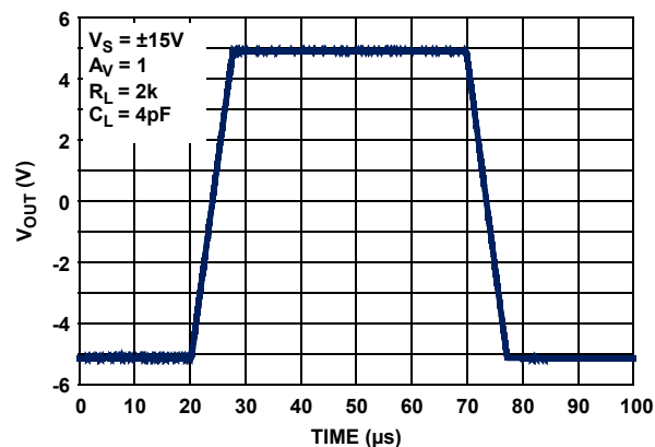
FIGURE 76. CHARACTERIZED LARGE-SIGNAL 10V STEP RESPONSE
