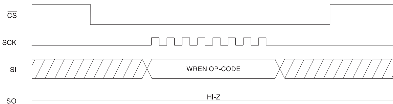
Figure 4-2. WREN Timing
