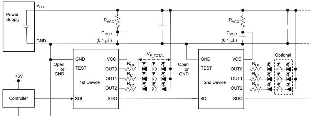
Figure 10. Internal Shunt Regulator Mode Application Circuit
