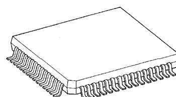
QFP60-P-1414-0.80E
