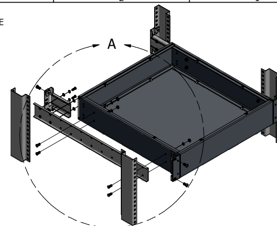
ISOMETRIC VIEW (EXPLODED)
