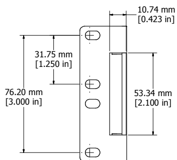
(1) REAR SUPPORT BRACKET FRONT VIEW
