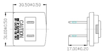
USA/CANADA PLUG
