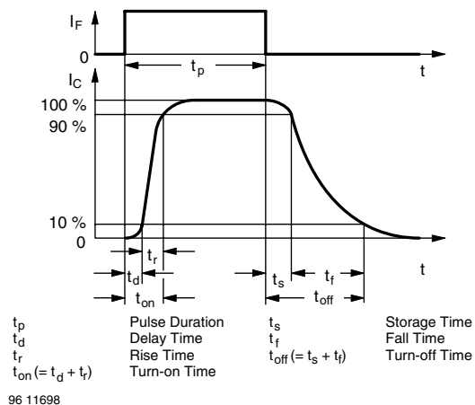
Fig. 3 - Switching Times
