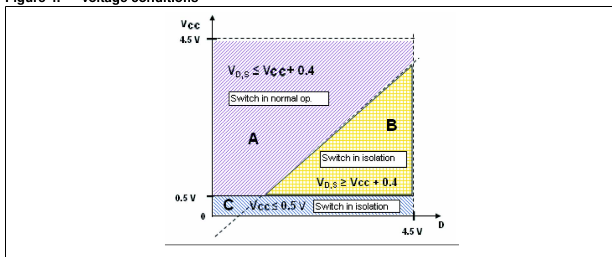
Figure 4. Voltage conditions
