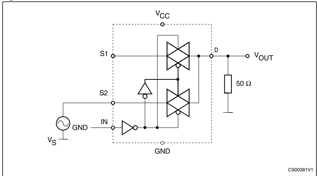
Figure 10. Test circuit
