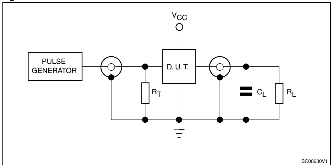
Figure 10. Test circuit
