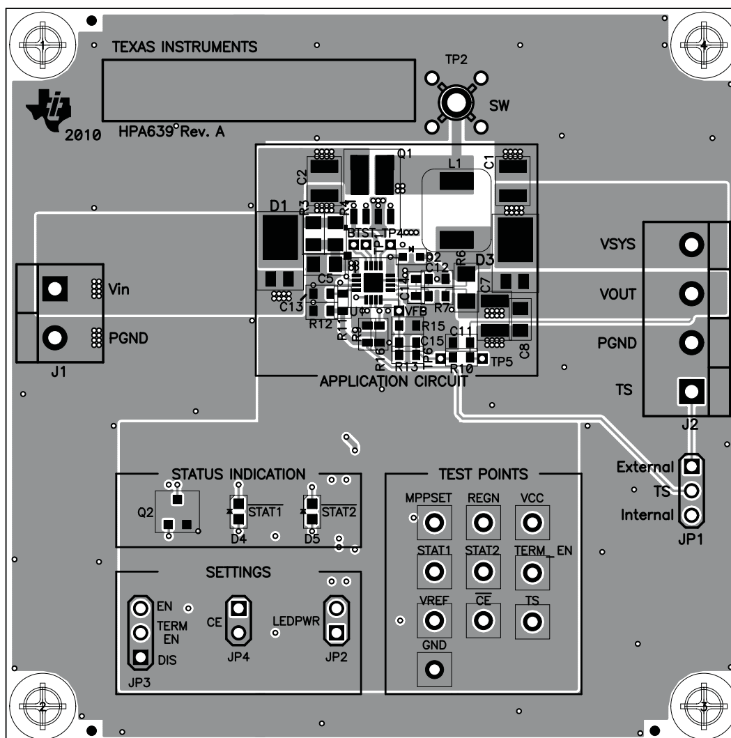
Figure 6. Top Assembly
