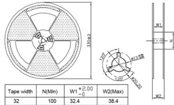
Figure 20: FT-X3 Reel and Hub Drawing
