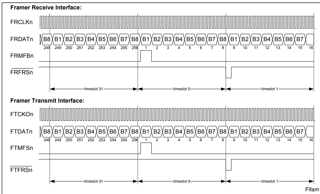
Figure 23 Framers Interface in FAM
