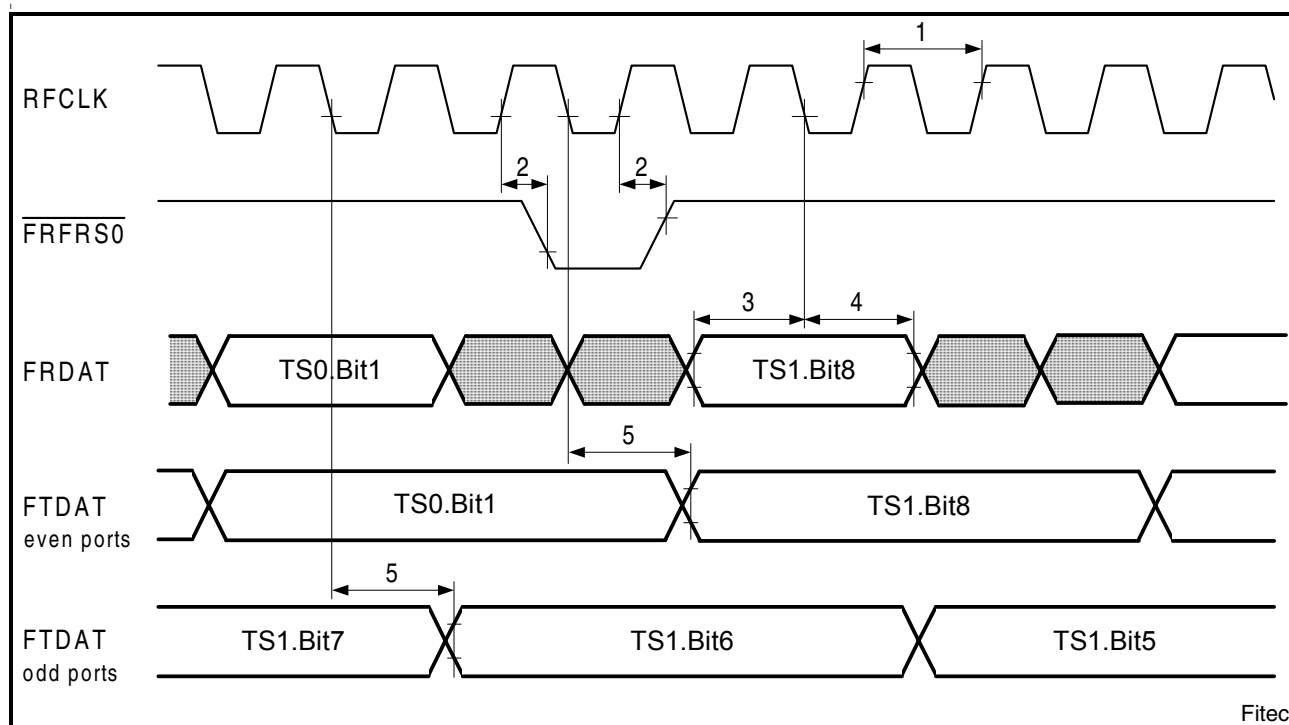
Figure 63 Framer Interface Timing in EC Mode
