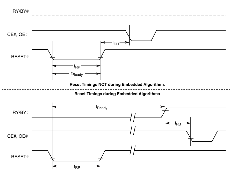
Figure 17.2 Reset Timings
