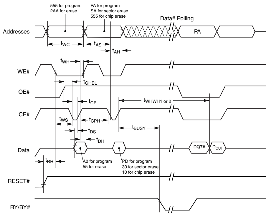
Figure 17.14 Alternate CE# Controlled Write (Erase/Program) Operation Timings
